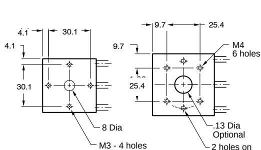
SERIES R300MM
