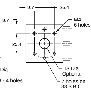
SERIES R450MM
