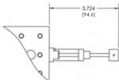
CENTER DRIVE 2" (50MM) LEAD SCREW
